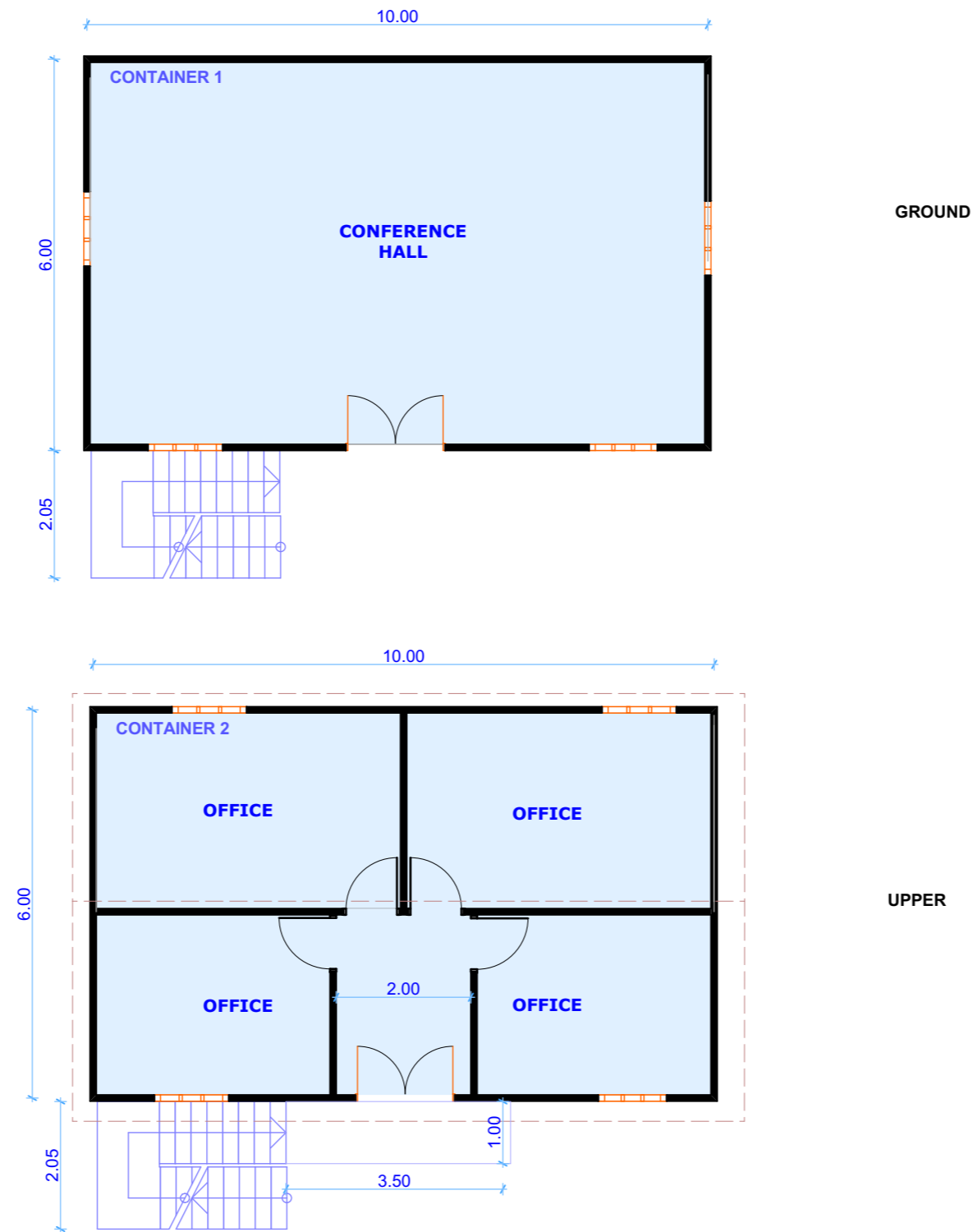
10X6.00 METERS PREFAB PLAN
